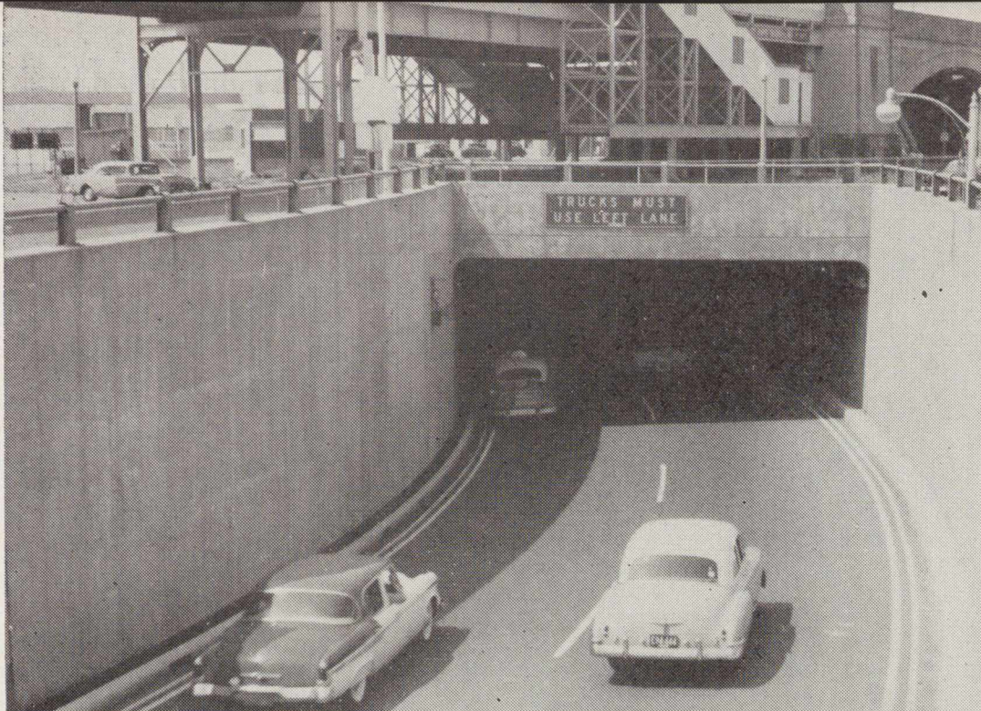
TUNELIS BOSTONE (Storrow Drive 1953 mt.). Projektavo inž. B. Galinis. BOSTON TUNNEL constructed from plans drawn up by Eng. B. Galinis. Foto V. Adomavičius
