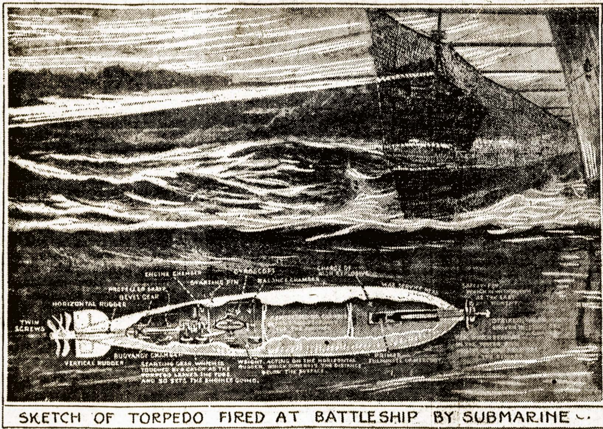
SKETCH OF TORPEDO FIRED AT BATTLESHIP BY SUBMARINE
