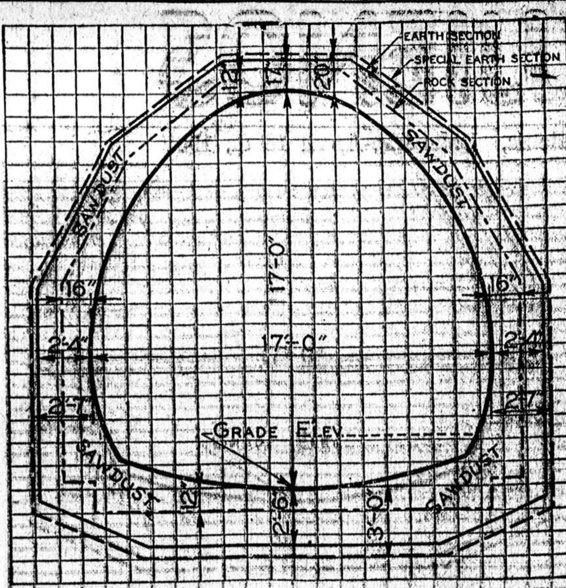
SANITARY DISTRICT TUNELIO SKERSPIUVIS
