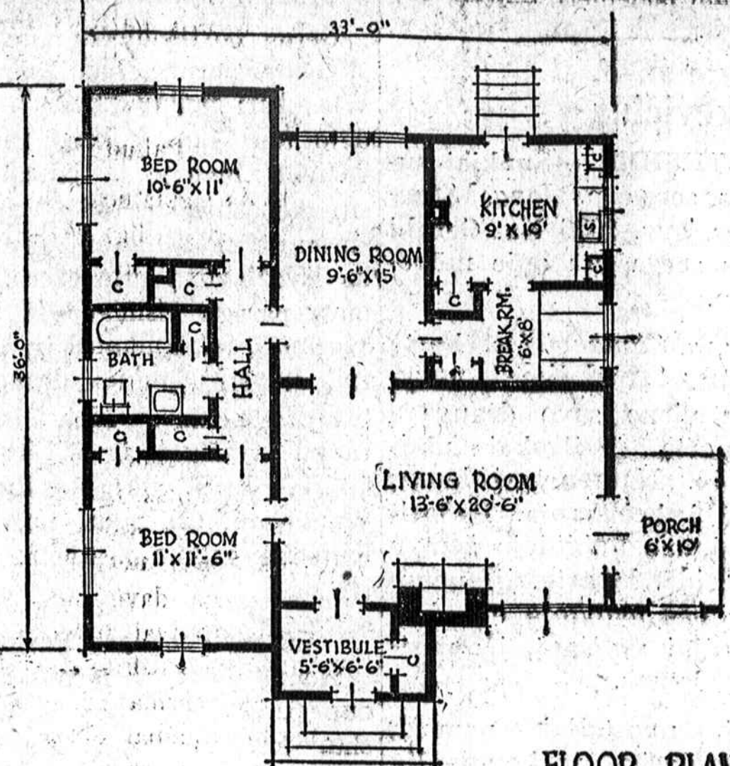
FLOOR PLAN
