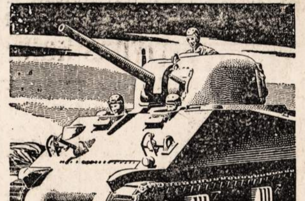
Gun mount cradles for tanks, formerly made of 27 parts, are made today at the Ford tank plant of only three castings, reducing production time by two-thirds and facilitating repairs in the field.
