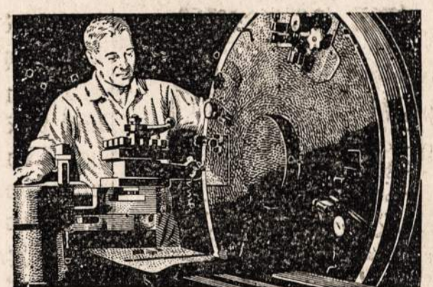
A horizontal engine lathe at Willow Run carrying Ford-designed equipment turns a gun-turret track for a B-24 Liberator. This machine saves time and holds the work to 1/10,000 of an inch.
