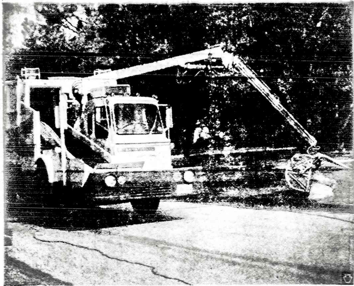
This new device for garbage collection promises to cut municipal costs while eliminating odors and insects and the noise normally associated with garbage collection. Called a Mechanical Bag Retriever (MBR), it is Gulf Oil Chemicals Company's entry into the $5 billion municipal refuse collection market. The MBR was developed by Bellaire, Texas, City Manager Tom Heffington, the inventor, and Gulf Oil Chemicals, a manufacturer of polyethylene garbage bags.
