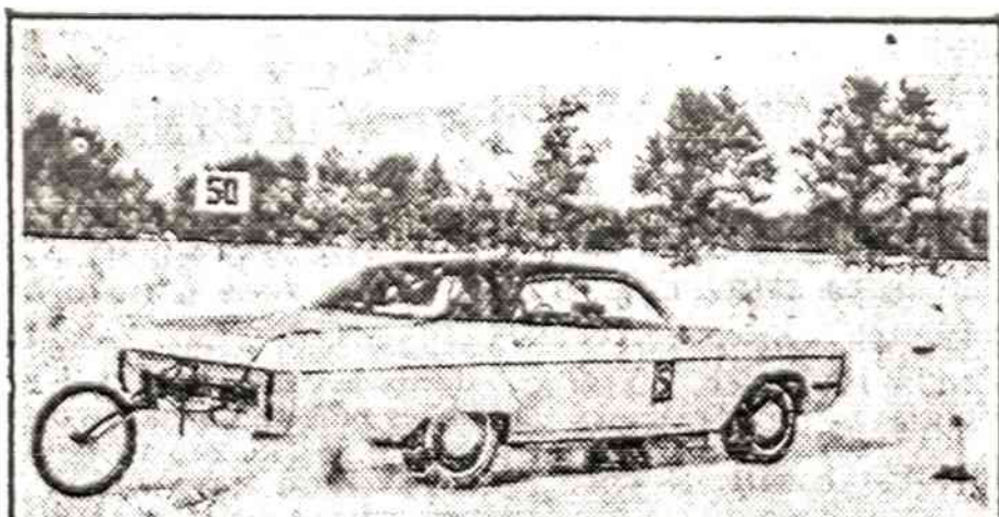
A test car brakes to a stop on glare ice during the National Safety Council's winter driving test program. Stopping ability of various types of tires, tire chains and other equipment are evaluated in the annual test program.
