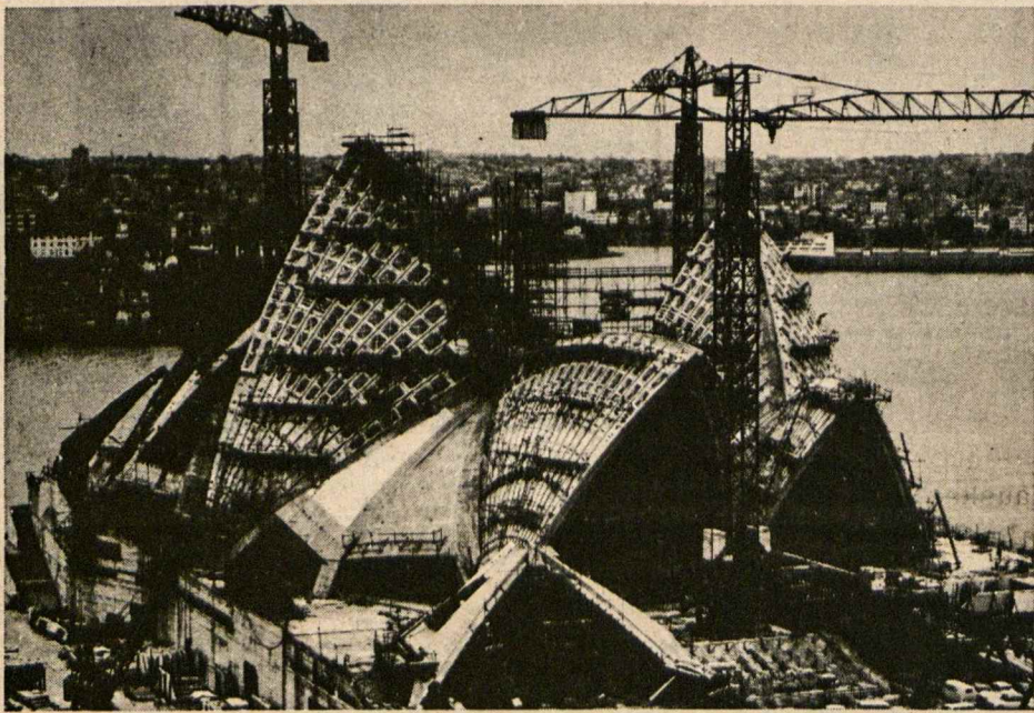
UTZON'S OPERA HOUSE (IN CONSTRUCTION) Setting sails in concrete.
