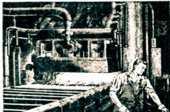
A new Ford method of quenching tank armor plate eliminates later straightening. Dies hold the plate during the process. Forty hours are saved on each M-4 medium tank and M-10 tank destroyer hull.
